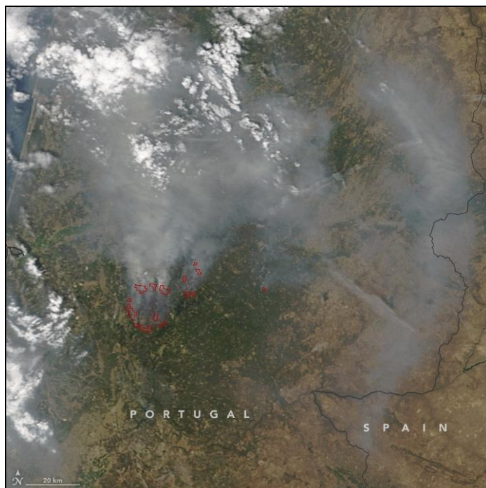
Figure 1. Satellite image of the fires in Portugal — June 18, 2017 (source: https://earthobservatory.nasa.gov/NaturalHazards/view.php?id=90423 )
