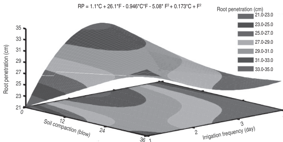
Figure 6. Surface chart of root penetration (RP) in contrast with soil compaction (C) and irrigation frequency (F)
