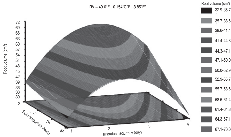
Figure 7. Surface chart of root volume (RV) versus soil compaction (C) and irrigation frequency (F)
