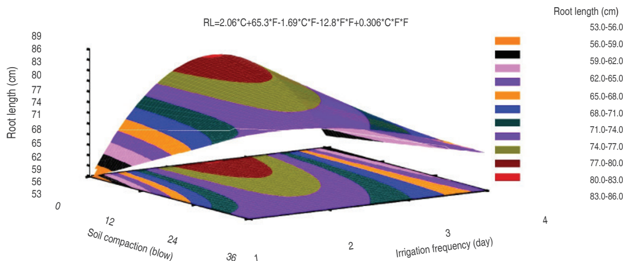
Figure 5. Surface chart of root length (RL) in contrast with soil compaction (C) and irrigation frequency (F).
