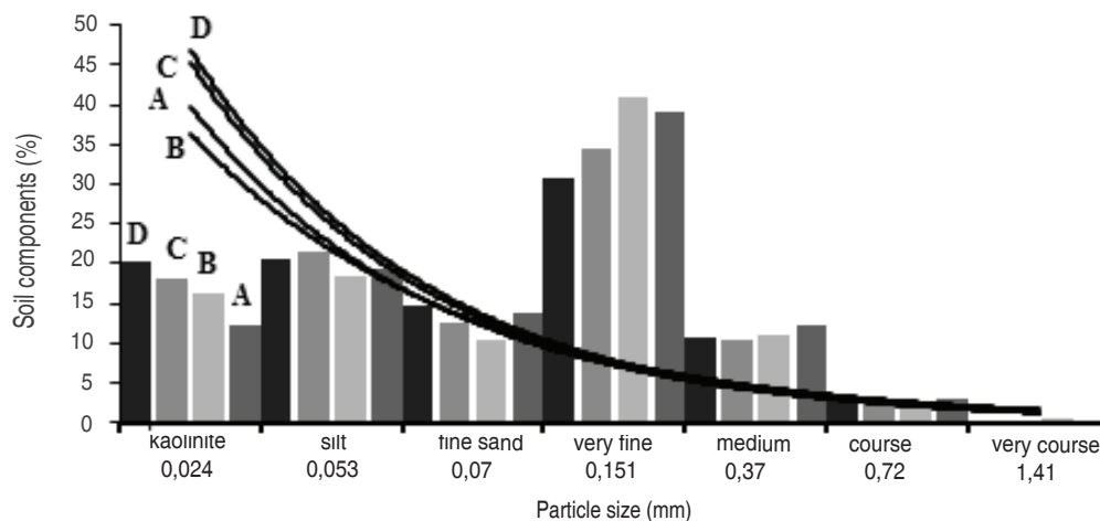
Figure 1. Soil components related to particle size in the four horizons studied. Particle trends size in contrast with depth (displayed with colors) are: (A) 0-15 cm, (B) 15 to 30 cm, (C) 30 to 45 cm and (D) 45 to 60 cm.
