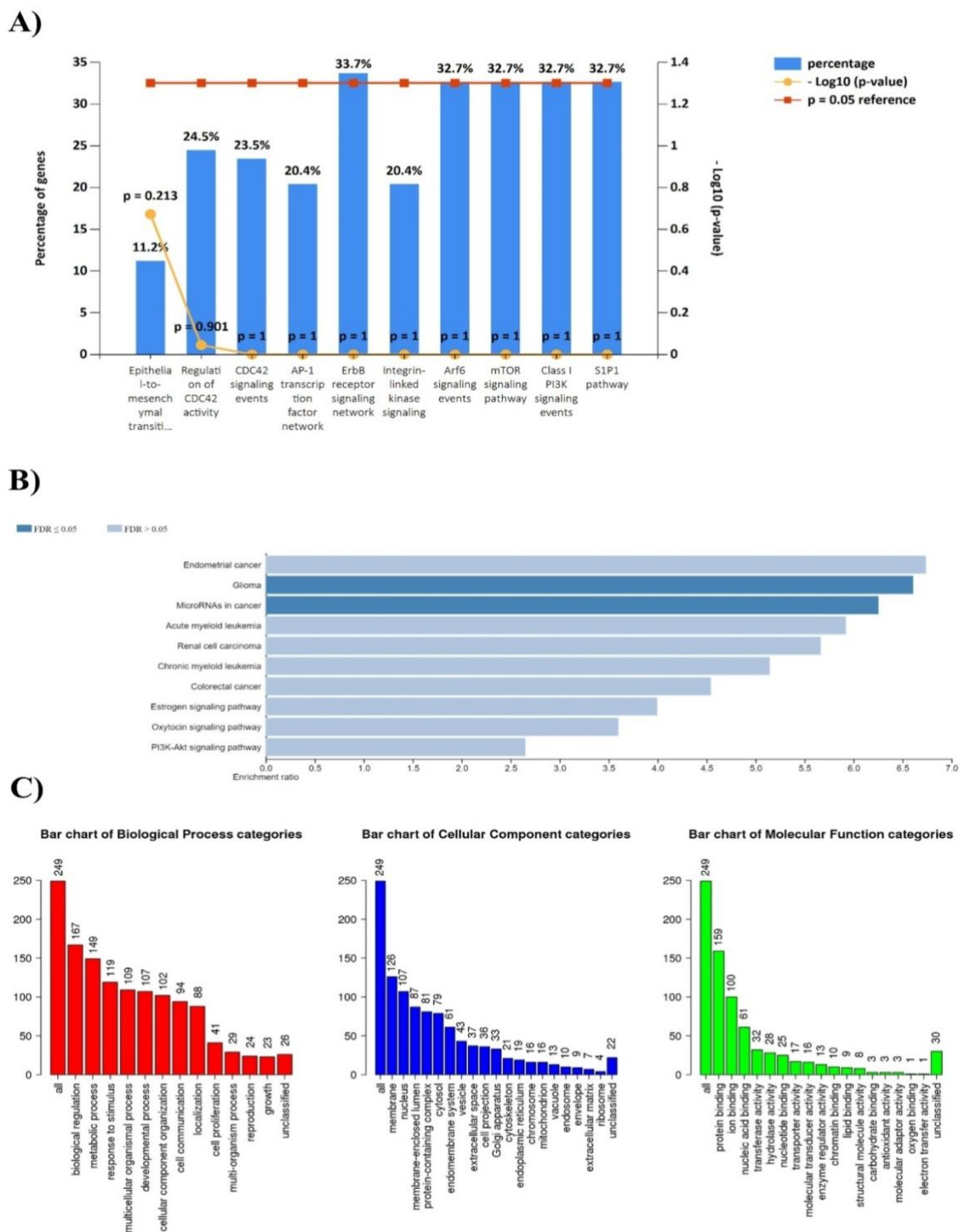
Figure 3. A) Biological pathways that were predicted from the target genes of three selected miRNAs using the FunRich tool. B) Enriched network of the same target genes using the Webgestaltweb-based tool. C) Gene ontology analysis of the target genes from the Webgestaltweb.
