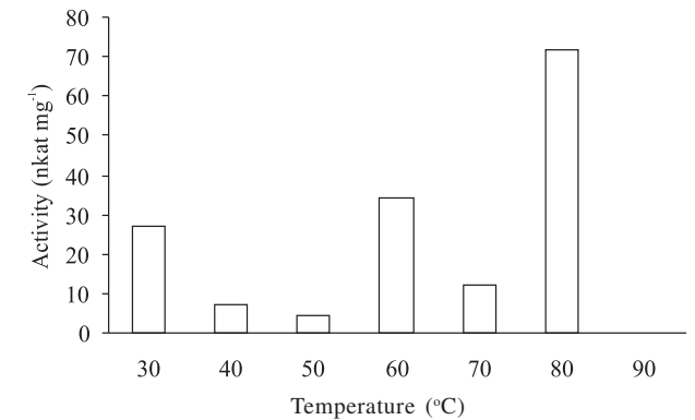
Fig 9 The effect of temperature on keratinase activity strain 45I-3 at pH 8.5.
