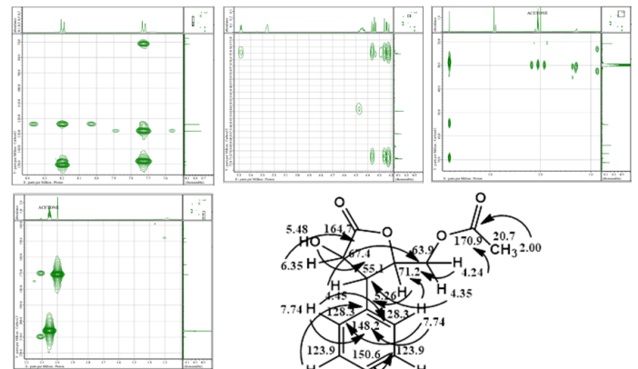
Figure 4. The HMBC spectra (A) and HMBC Correlation (B) of Compound 1
