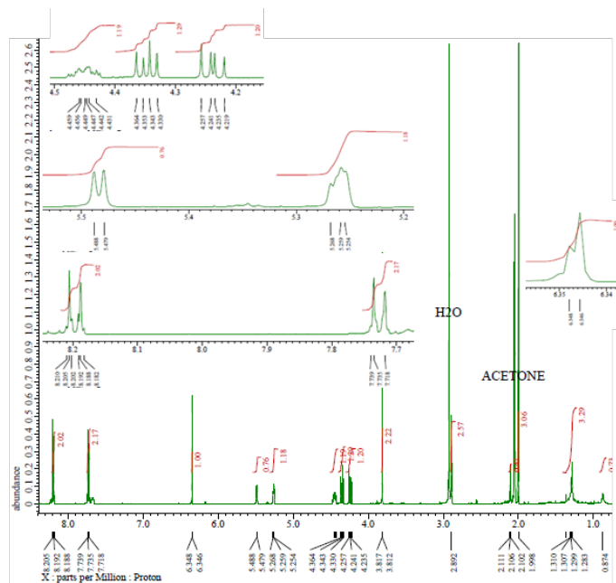
Figure 2. The 1 H-NMR spectra of compound 1
