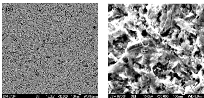
Fig 4. SEM of the samples of films with a thickness of 140 nm (a) and 1 \mu\text{m} (b), obtained by electrodeposition for 30 min at a current density of 0.5 (a) and 3 \text{mA cm}^{-2} (b) with subsequent annealing at 773 K.
