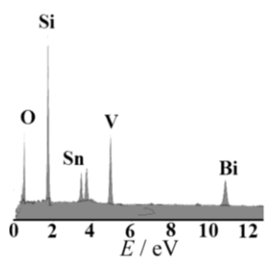
Fig. 3. EDAX spectrum of \text{BiVO}_4/\text{SnO}_2 electrode elements.
