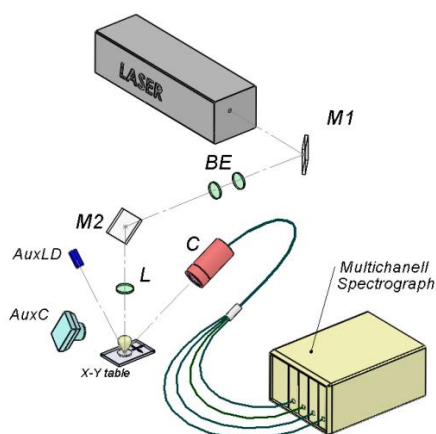
Fig. 1. Experimental setup. M1 and M2 are bending mirrors; BE is beam expander; L is focusing lens; AuxC is video-camera, AuxLD is pointing red diode laser ( \lambda = 635 nm), and C is an optical system for the signal collection.
