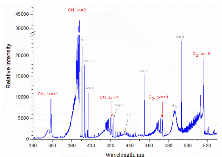
Fig. 5. Part of the time-integrated LIBS spectra of Oil-100 sample showing characteristic emission bands of C_2 and CN molecules.
