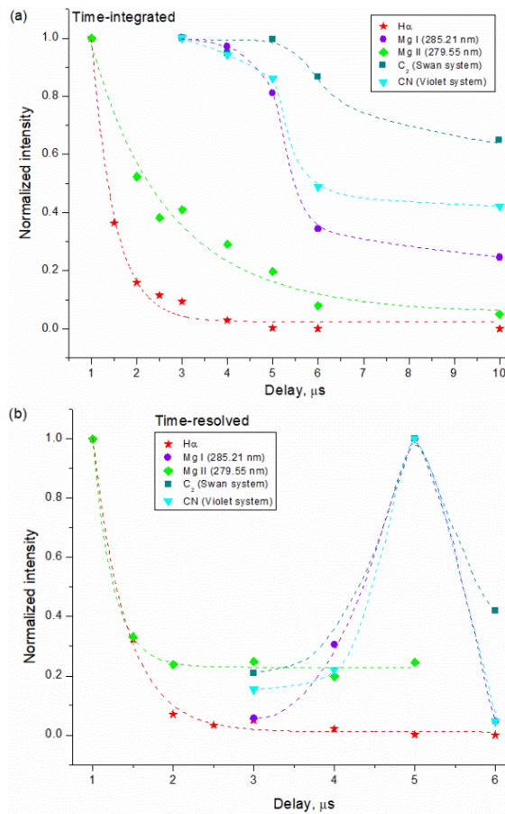
Fig. 2. Spectral line emission intensity of various species in plasma of Oil-100 as a function of time from the laser pulse: a) Time-integrated values and b) calculated time-resolved values, equivalent to the integration time of 1 \mu\text{s} .
