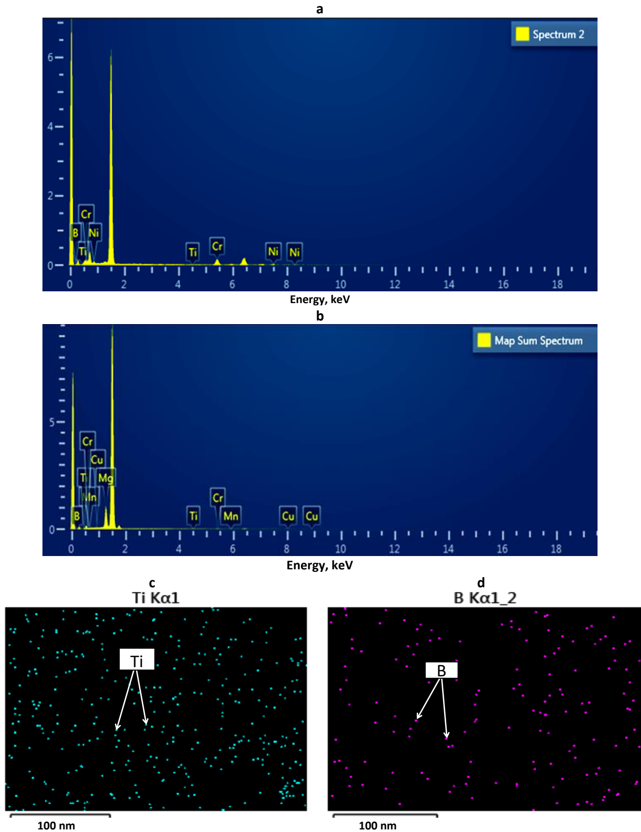
Figure 2. EDS of composite specimens (a) AA6061 + 5 vol.% \text{TiB}_2 ; (b) AA6061 + 10 vol.% \text{TiB}_2 ; Layered EDS image for (c) Ti and (d) boron
