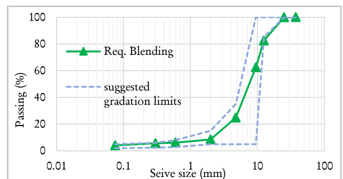
Figure 2: Aggregate gradation curve in comparison with suggested limit curves
