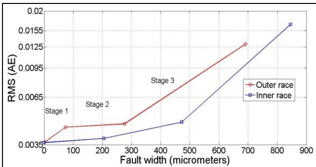
Figure 16. RMS values for inner and outer race bearing faults regarding different levels of severity
