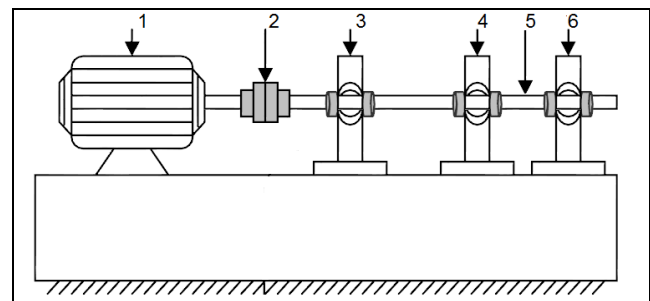
Figure 2. Test bench
