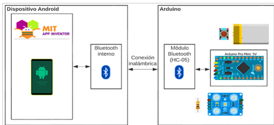
Fig. 4. Schematic of the application architecture
