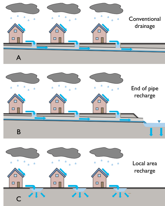
Fig. 2. Three model scenarios for stormwater drainage infrastructure.
