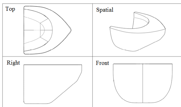
Figure 4. Module icebreaker shapes
