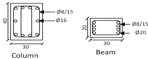
Fig. 3. Reinforcement details of the studied structure.
