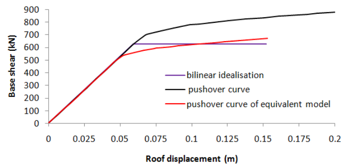
Fig. 5. Pushover curves and bilinear idealization.
