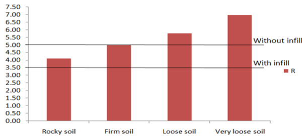
Fig. 13. Behavior coefficient without SSI (N2).
