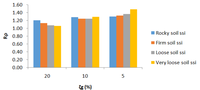
Fig. 12. R_p VS \zeta_g\% and soil type.
