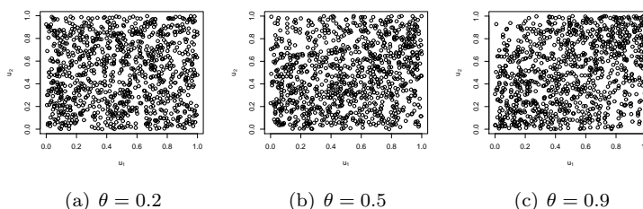
FIGURE 4: Plots of data under different FGM dependence structures.
