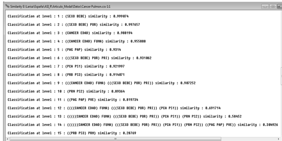
FIGURE 5: Classes and similarity indexes obtained by executing CHIC.
