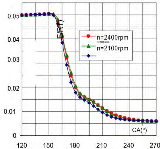
Figure 12. Variation of X_f \cdot \exp(-E/RT) in function of crank angle with different engine speeds (D20, \phi=1 )
