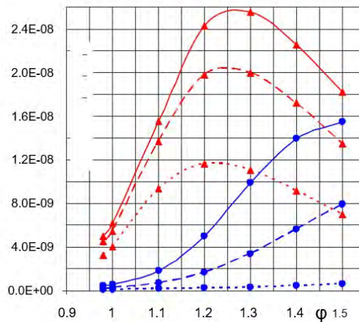
Figure 11. S_{max} ( \blacktriangle ), S_{exhaust} ( \bullet ) vs equivalence ratio with different diesel content in the fuel ( \bullet : D25, \blacktriangle : D20, \circ : D15, n=2400rpm)
