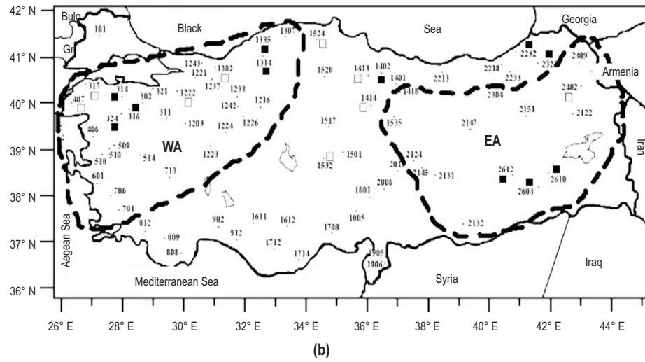
Figure 4. Population differences for the hypothetical and original streamflow series for (a) Scenario C and (b) Scenario D. Solid (open) squares represent the 95% (90%) significance level.
