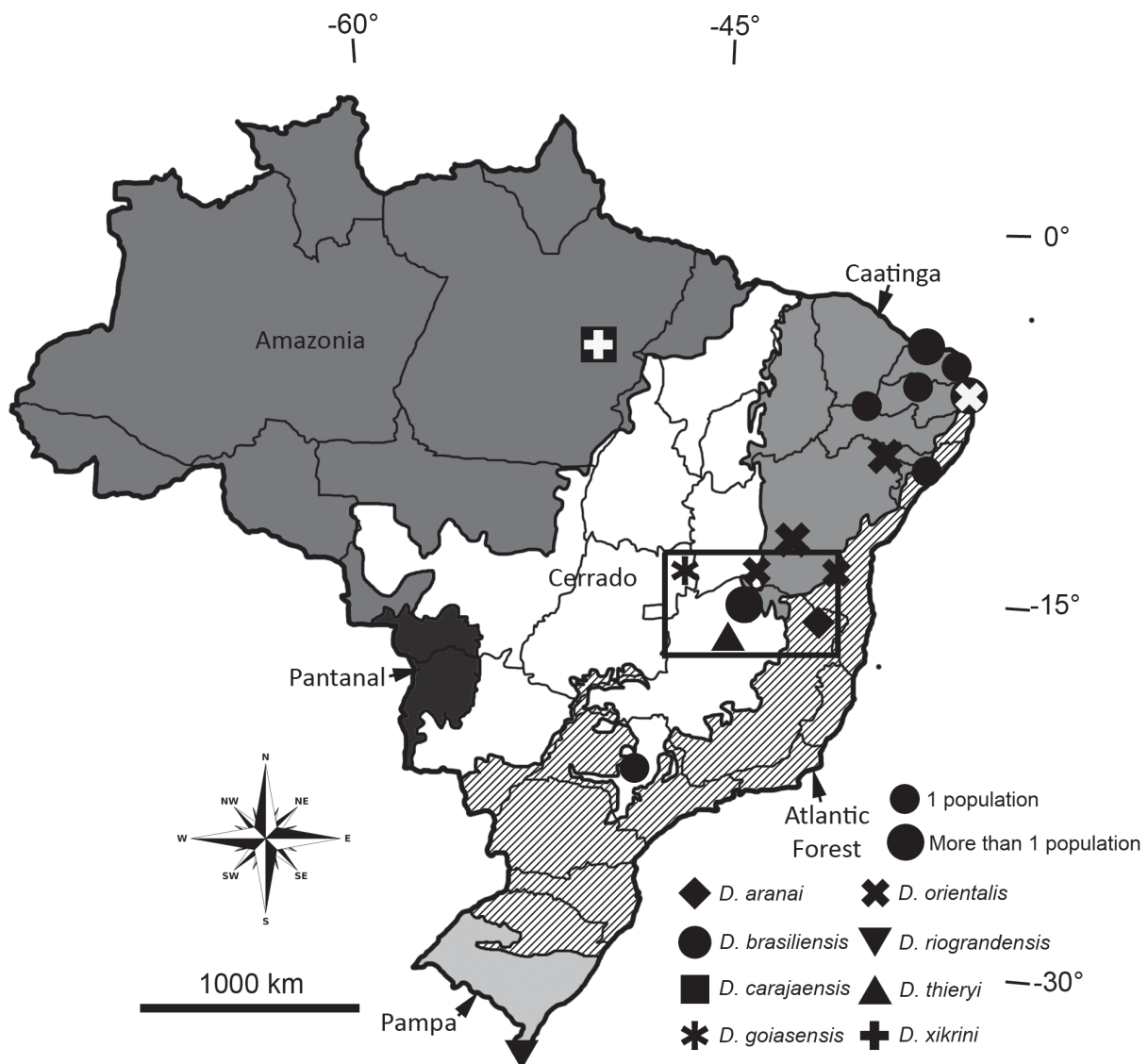
Fig. 1. Distribution of Brazilian Dendrocephalus Daday, 1908. The main biomes are indicated on the map, the empty black square delineates the hotspot of richness of Dendrocephalus in Brazil. The symbols are black except in the case of sympatry, where one of the species is in white.
