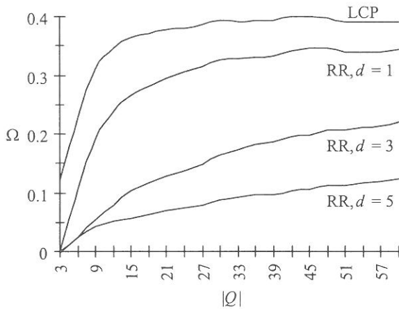
Fig. 1 Cost effectiveness of the re-routing ( |V| = 60 , \bar{e} = 5 , \alpha = 0.25 , k = 3.5 ).
