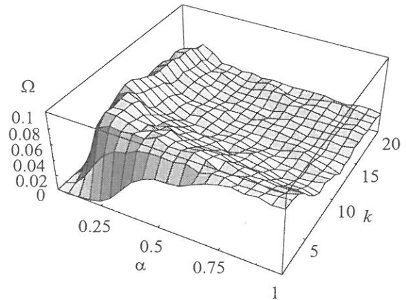
Fig. 3 Influence of the network density on the cost effectiveness of the stable tree ( |V| = 60 , |Q| = 15 , d = 3 , \bar{e} = 5 ).
