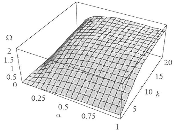
Fig. 4 Influence of the network density on the cost effectiveness of the initial tree ( |V| = 60 , |Q| = 15 , d = 3 , \bar{e} = 5 ).
