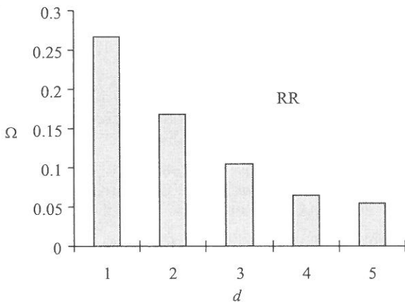
Fig. 2 Impact of the search diameter on cost effectiveness ( |V| = 60 , |Q| = 15 , \bar{e} = 5 , \alpha = 0.25 , k = 3.5 ).
