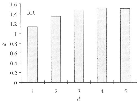
Fig. 5 Average number of parallel transitions ( |V| = 60 , |Q| = 15 , \bar{e} = 5 , \alpha = 0.25 , k = 3.5 ).
