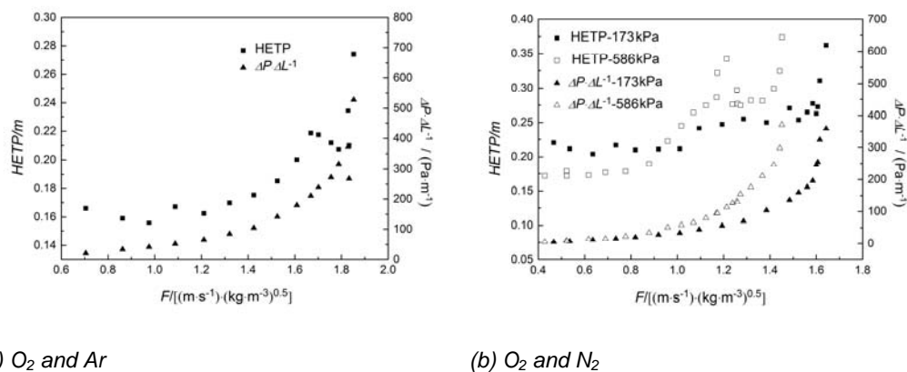
Figure 4: HETP and pressure drop for SCFP-SiC in air separation system
