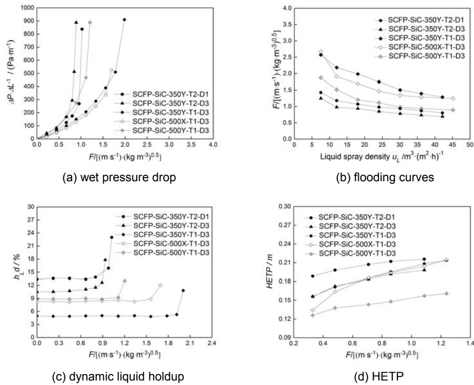
Figure 3: main performance parameters for SCFP-SiC with different specific area, corrugation angle, foam diameter and corrugated thicknesssheet thickness
