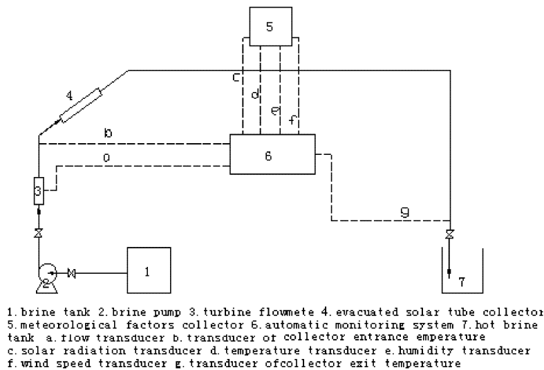
Fig.1 Brine solar energy heating experimental setup
