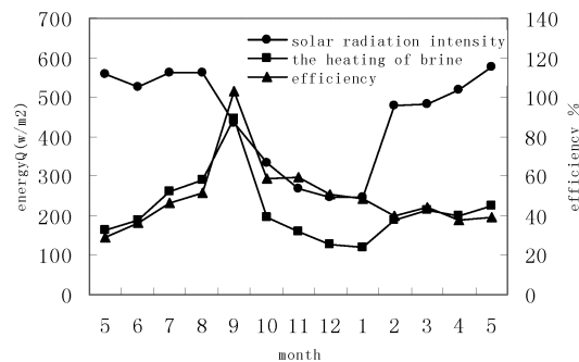
Fig.3 Solar radiation intensity, the heating of brine and the efficiency change
