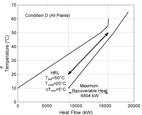
Figure 5. Composite curves showing indirect heat transfer between plants using HRL for condition D.
