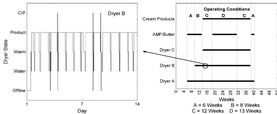
Figure 3. Semi-continuous operation of Dryer B (left) and a representative operating schedule (right) indicating the four operating conditions of the factory.
