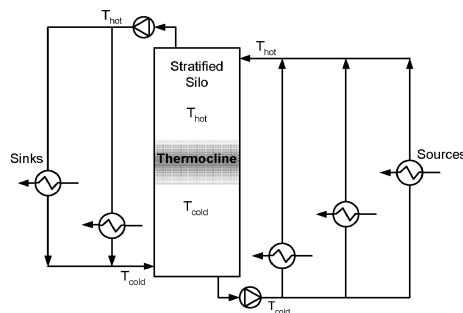
Figure 4. Schematic of the heat recovery loop including a stratified tank.
