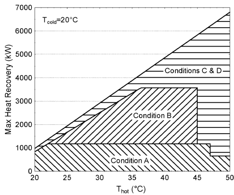
Figure 6. Effect of T_{hot} on maximum heat recovery for the several operating conditions.
