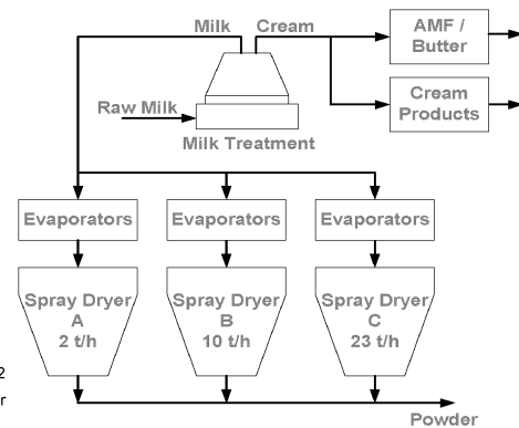
Figure 2. Schematic of the dairy factory with the five separate plants.
