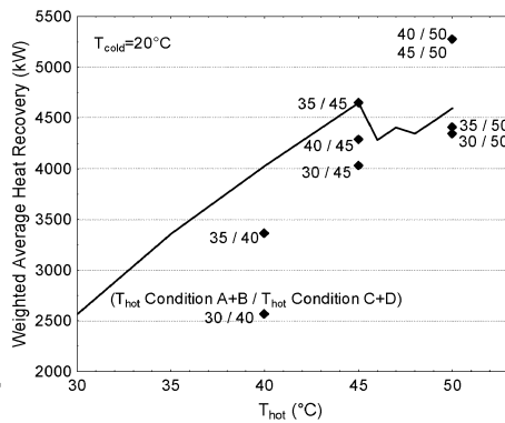
Figure 7. Weighted average heat recovery for all conditions with split HRL operating scenarios.
