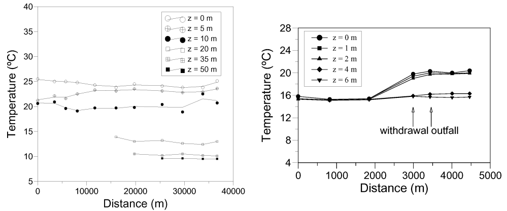
Fig.2. a) Stratified big reservoir (Entrepeñas). b) Stratified small reservoir (Zorita)
