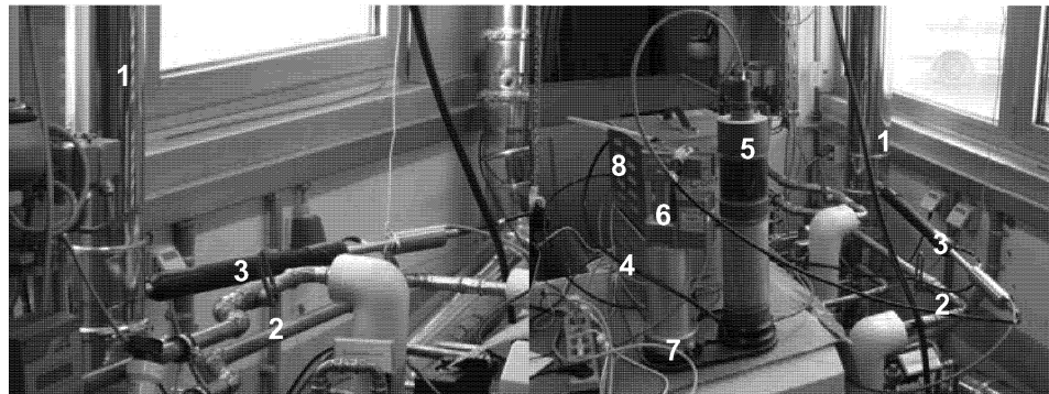
Figure 2: Left: Sampling probe of the emission sampling system (ESS) connected to the stack. Right: Complete setup consisting of sampling probe, dryer and filter for dilution air, control unit and SMPS+E for particle analysis. Legend: 1: Stack with exhaust gas, 2: Hydraulic connection and sensors, 3: Sampling probe, 4: Control unit, 5: Dryer and filter for dilution air, 6: M-DMA, 7: FCE, 8: DMA Controller
