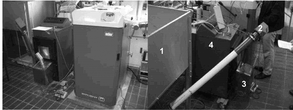
Figure 1: Left: Pellet burner (blue) and wood gas burner (red) in the laboratory of Dezentrale Energiesysteme at the institute for energy technique and motion technique, University of Applied Science, Ulm. Right: Pellet burner with pellet storage and auto feeding system. Legend: 1: Storage for wood pellets, 2: Electrical auto feeding system, 3: Pellet burner with control unit and housing, 4: Burner, adapted for experimental use, originally a simple wood burner.
