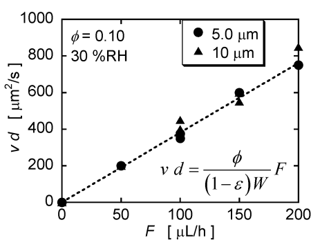
Figure 5: Effect of particle diameter of feed suspension on coating speed using 5.0 or 10 \mu\text{m} diameter of PSL.
