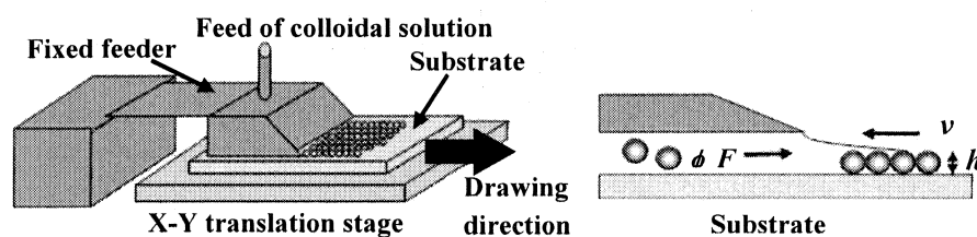
Figure 1: schematic diagram of the continuous coating method and definition of operation parameters.
