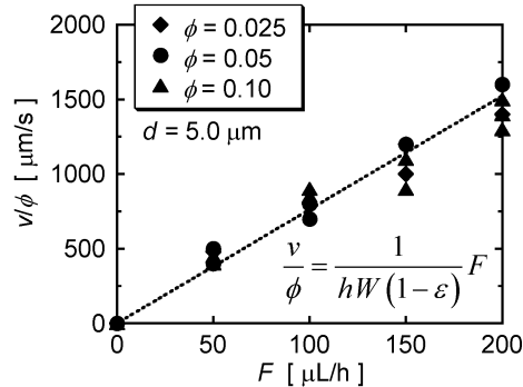
Figure 6: Effect of particle volume fraction of feed suspension on coating speed using 5.0 \mu\text{m} diameter of PSL.
