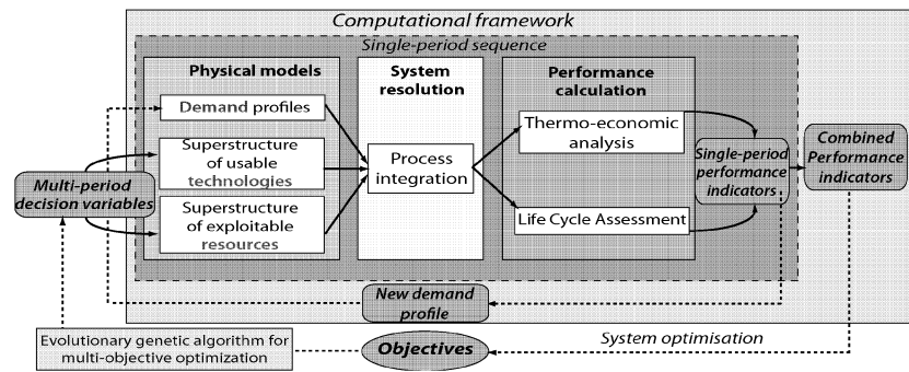
Figure 1: Computational framework
