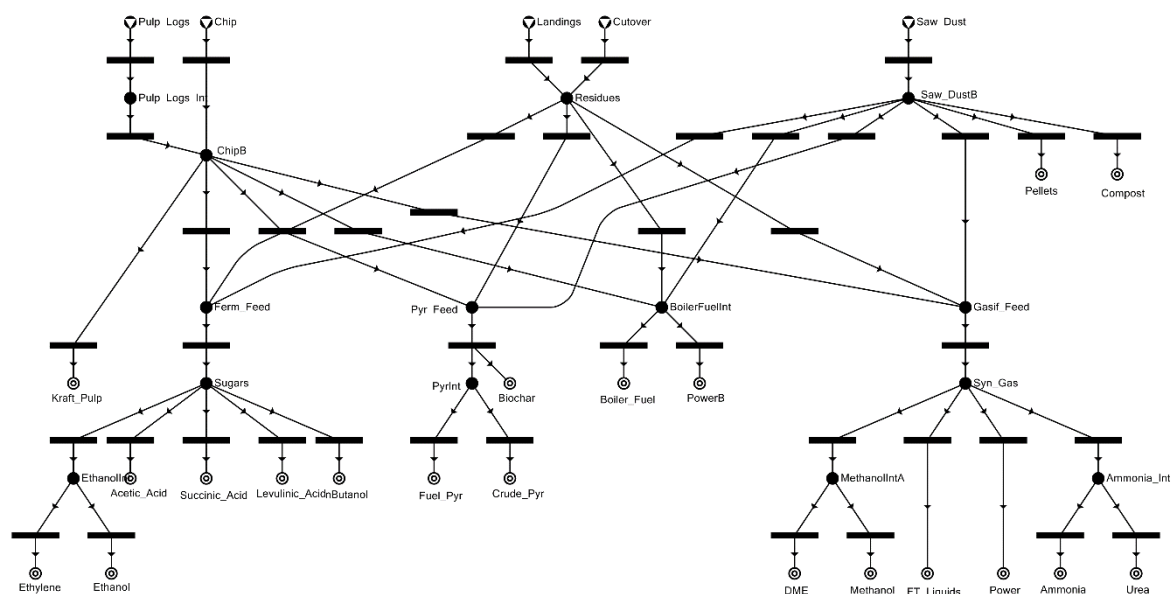
Figure 1: Maximal structure of the P-graph for the processing of process and forest biomass residues
