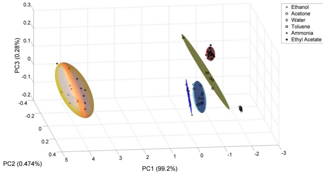
Figure 4: PCA plot for e-nose 1
