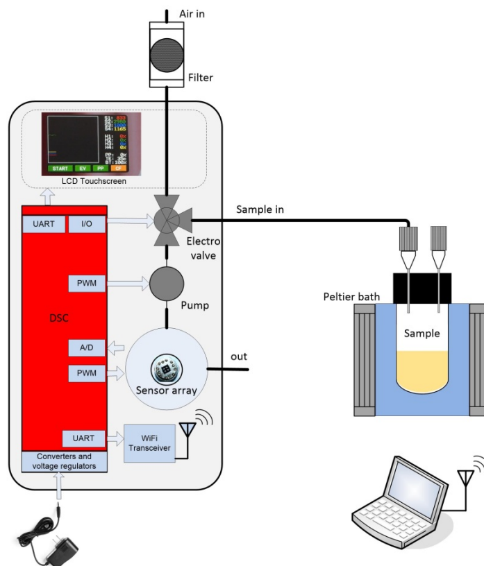
Figure 3: Schematics of the e-nose and the measurement setup.
