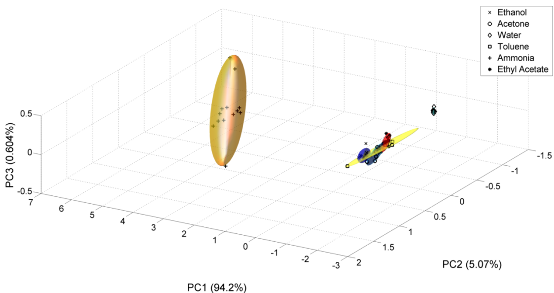
Figure 5: PCA plot for e-nose 2
