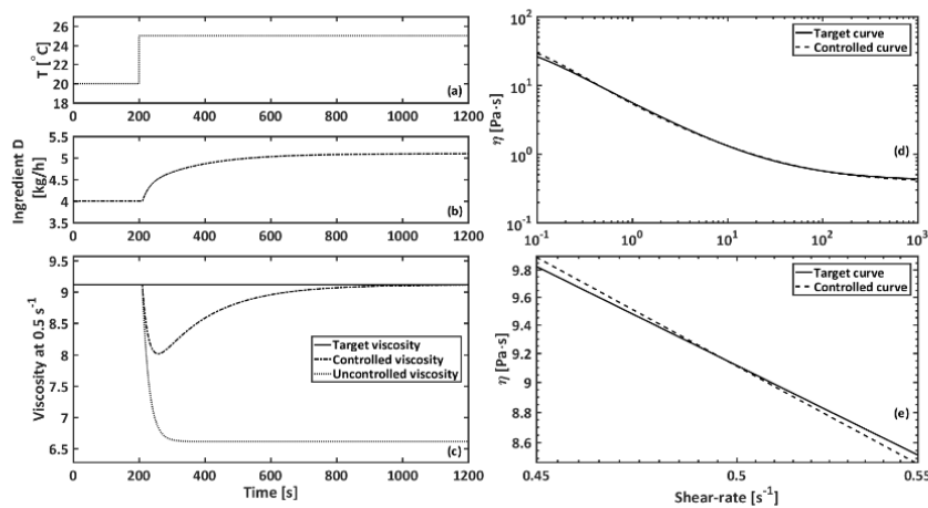
Figure 5: Controlled system responses
