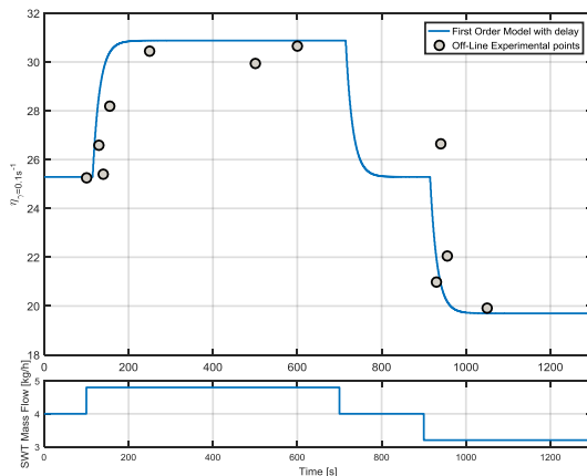
Figure 4: Prediction of the empirical model (solid line) compared with experimental points (full circles) in presence of a 20% step-test variation in the D ingredient flow feed
