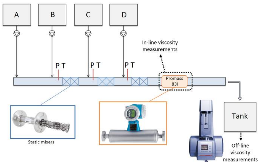
Figure 1: Scheme of the process
