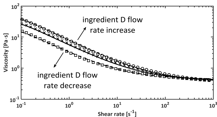
Figure 3: Rheological behavior of the detergent at different process conditions.
