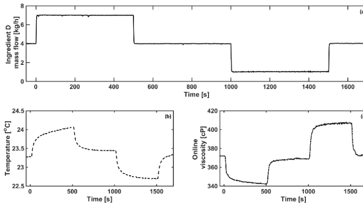
Figure 2: Step variation of the ingredient D flow and output responses of temperature and online viscosity.
