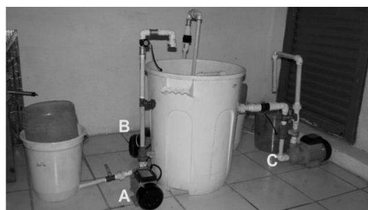
Figure 2: Comparison between the illustrative and real systems from The Oil Cage with the biosurfactant (A), oil, and mixture (C) pumps
