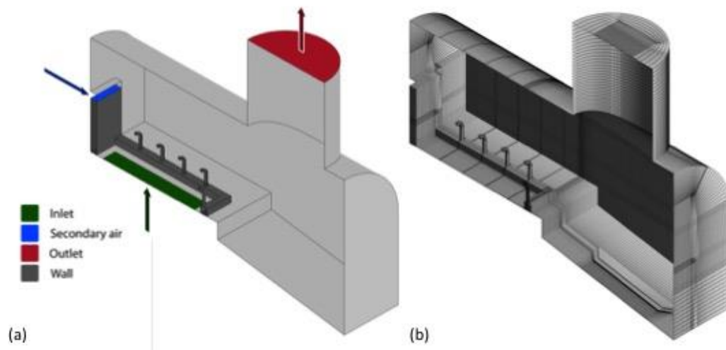
Figure 3: Computational domain (a) and grid (b).
