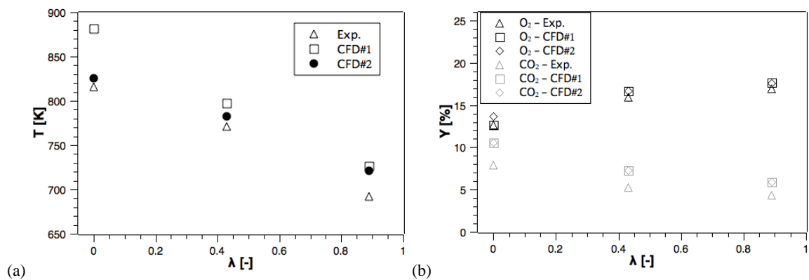
Figure 4: Comparison between experimental measurements of (a) temperature, (b) O_2 and CO_2 mass fractions and those predicted with the CFD model #1 and #2 for different secondary to primary air flow ratios.
