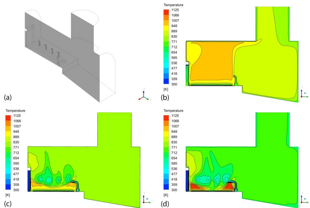
Figure 6: Distribution of temperature on the boiler symmetry (a) predicted with CFD model #2 at different secondary to primary air flow ratios: (b) \lambda=0 , (c) \lambda=0.43 , (d) \lambda=0.89 .
