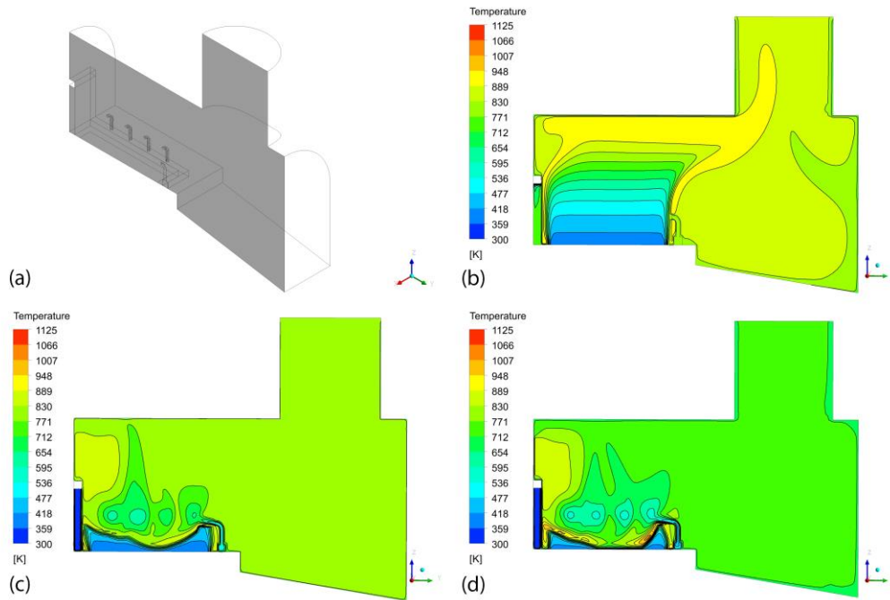
Figure 5: Distribution of temperature on the boiler symmetry (a) predicted with CFD model #1 at different secondary to primary air flow ratios: (b) \lambda=0 , (c) \lambda=0.43 , (d) \lambda=0.89 .
