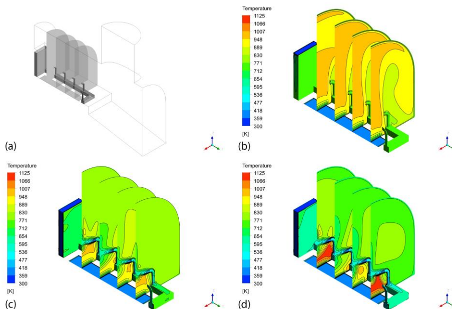
Figure 7: Distribution of temperature at different cross sections in the boiler (a) predicted with CFD model #2 at different secondary to primary air flow ratio: (b) \lambda=0 , (c) \lambda=0.43 , (d) \lambda=0.89 .
