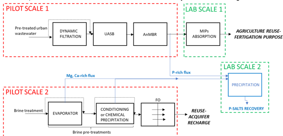
Figure 1: Overall concept for non-conventional water sources use and P-recovery
