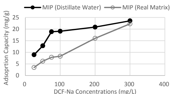
Figure 4: Adsorption tests performed on MIPs at different concentration of DCF-Na in AnMBR permeate
