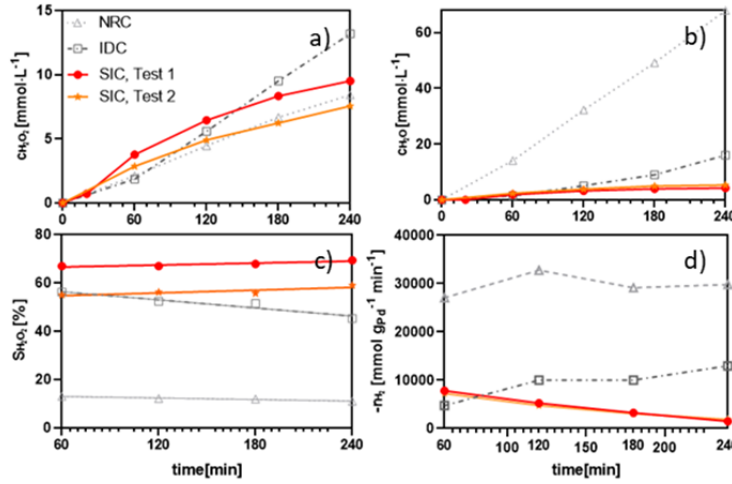
Figure 2: Comparison of the SIC with IDC and NRC catalysts (Abate et al., 2016) with respect to a) the formation of H_2O , b) H_2O_2 , c) H_2O_2 selectivity, and d) H_2 consumption rate ( r_{H_2} ) as a function of time.
