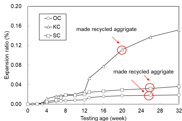
FIGURE 4. Expansion test on monitoring specimens.
