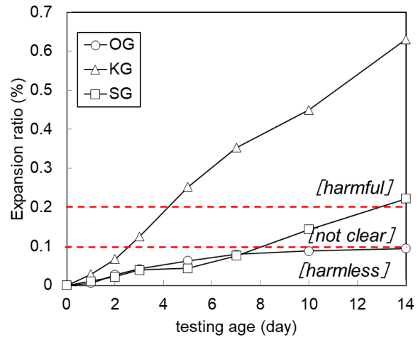
FIGURE 2. Accelerated mortar bar test on ASTM.
