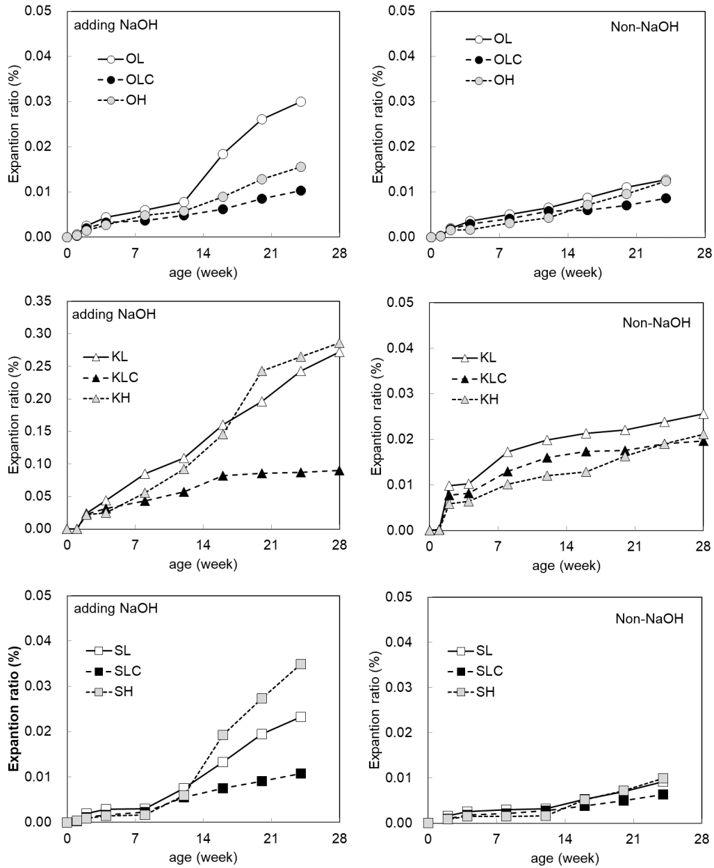
FIGURE 6. Results of re-ASR on recycled concrete.
