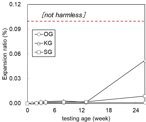
FIGURE 1. Mortar bar test on JIS.
