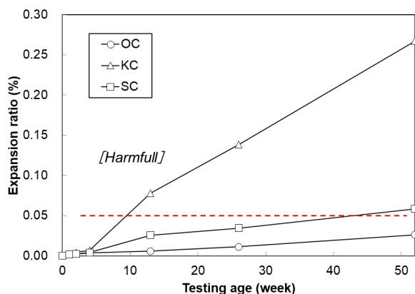
FIGURE 3. ASR expansion test on RILEM.
