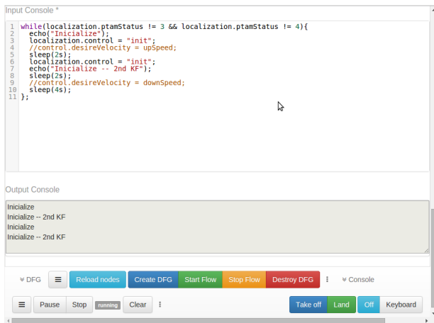
FIGURE 3. Urbiscript console. On the top – script editor, middle – output of executed script, bottom left – script execution control (surrounded with other controls of X-Copter Studio).
