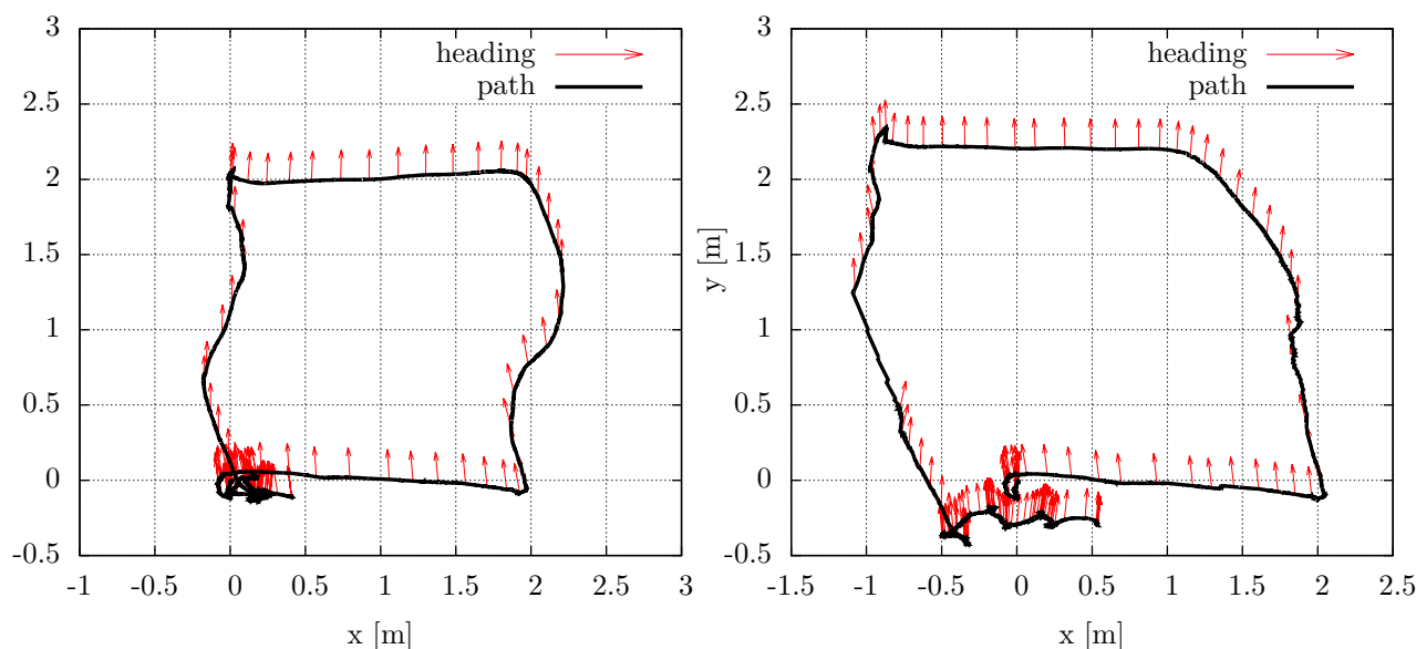
FIGURE 4. Example of a path tracked by the EKF. A square 2\text{ m} \times 2\text{ m} was set up and quadcopter was navigated (with PID controller) to its vertices using inertial localization only. Supposed position is shown on the left plot. As you can see, plot on the right shows more realistic pose and position thanks to visual localization (applied to the original data). Alas, we don't have any reference data for absolute comparison.
