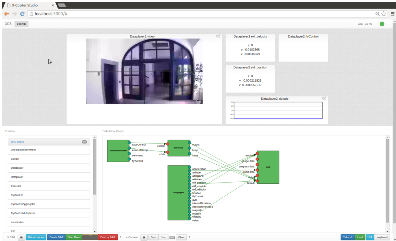
FIGURE 2. X-Copter Studio GUI. Top navbar indicated connection quality, upper half is filled with widgets that display data from the onboard, lower half accommodates the editor with repository of nodes on the left, and connected nodes on the right. At the bottom there are (left to right): dataflow control buttons, scripting console control buttons and manual flight control buttons. The scripting console is hidden.
