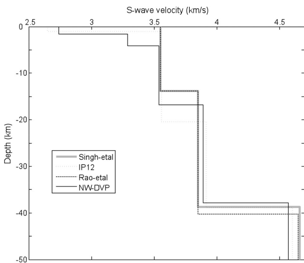
Figure 2. S-wave velocity structure of the Indian Peninsula in various studies: Singh-etal [Singh et al. 1999], IP12 [Bhattacharya 1992], Rao-etal [Rao et al. 2002], northwestern DVP [Prajapati et al. 2011]. Theoretical group velocity curves have been drawn in Figure 3 for these structures. IP12 is modified from IP11 [Bhattacharya 1981, 1992], whose top 1 km is replaced by a Deccan trap layer.
