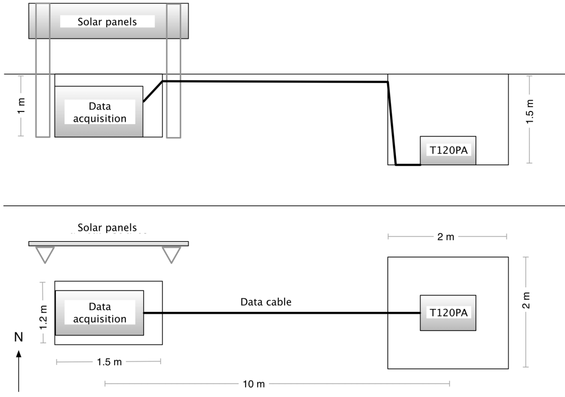
Figure 7. Installation configuration for the CASE-IPY profile stations, indicating the orientation and relative positions of the different components (top: side view; bottom: view from above).
