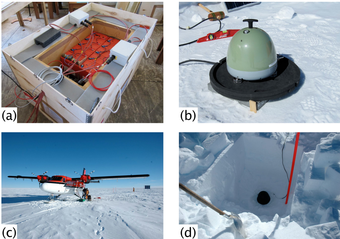
Figure 8. Deployment of the CASE-IPY profile stations. (a) Pre-installation test of the data acquisition box. (b) Pre-deployment test of the Trillium 120PA seismometer. (c) Field deployment with Twin Otter. (d) Seismometer in field pit before the installation of the protective box.
