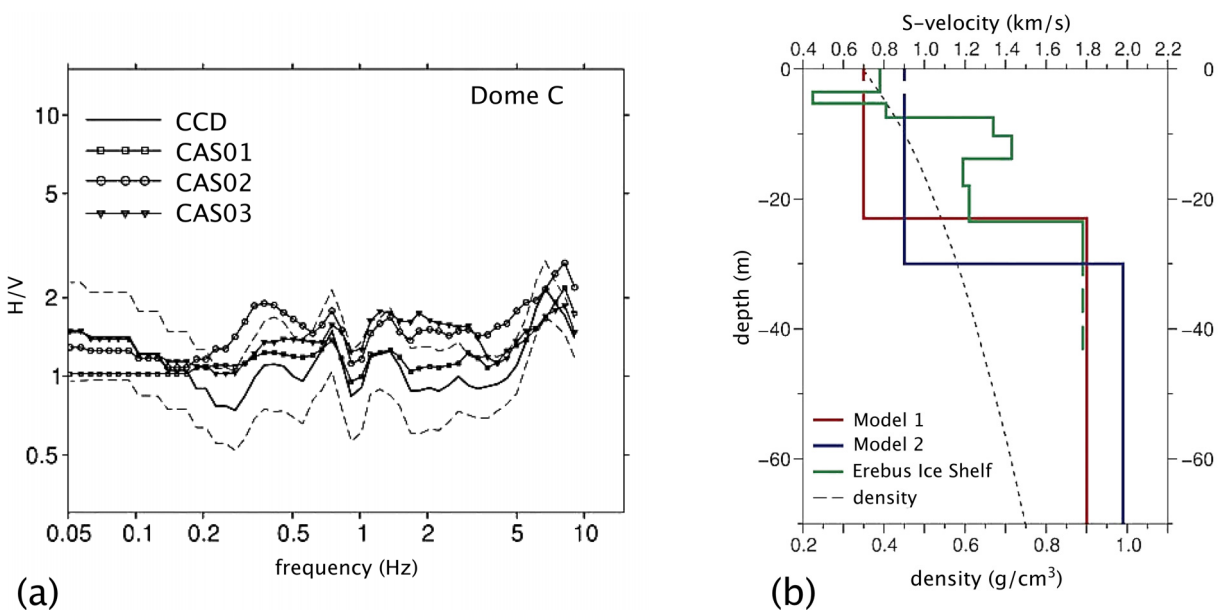
Figure 9. Snow structure at Dome C (after L ev eque et al. [2010]). (a) Mean spectral ratios of horizontal to vertical motion determined from noise at the four Dome C stations. The 1-sigma confidence level is similar for the different curves, and is shown for CCD only (dashed line). (b) S-wave velocity models. Model 1 is preferred, as it is the most compatible with the density profile at Concordia (L. Arnaud, personal communication 2010).
