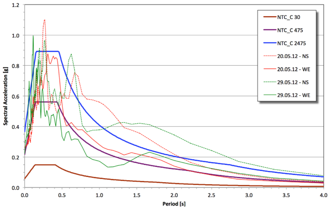
Figure 7. Comparison between the horizontal acceleration response spectra recorded at the MRN station for the two main events of the Emilia sequence, and the design code spectra prescribed by NTC08, for soil type C, for 30, 475 and 2475-year return periods (as indicated).
