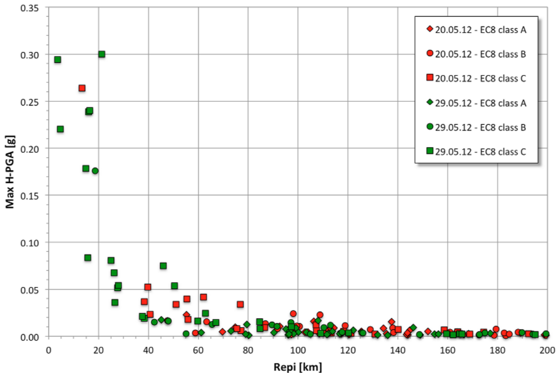
Figure 5. Larger horizontal PGAs (in g) versus the epicentral distance recorded for the May 20 and 29, 2012, earthquakes. The EC8 [CEN 2004] soil class of each station (as assigned based on the geological map) is also indicated.
