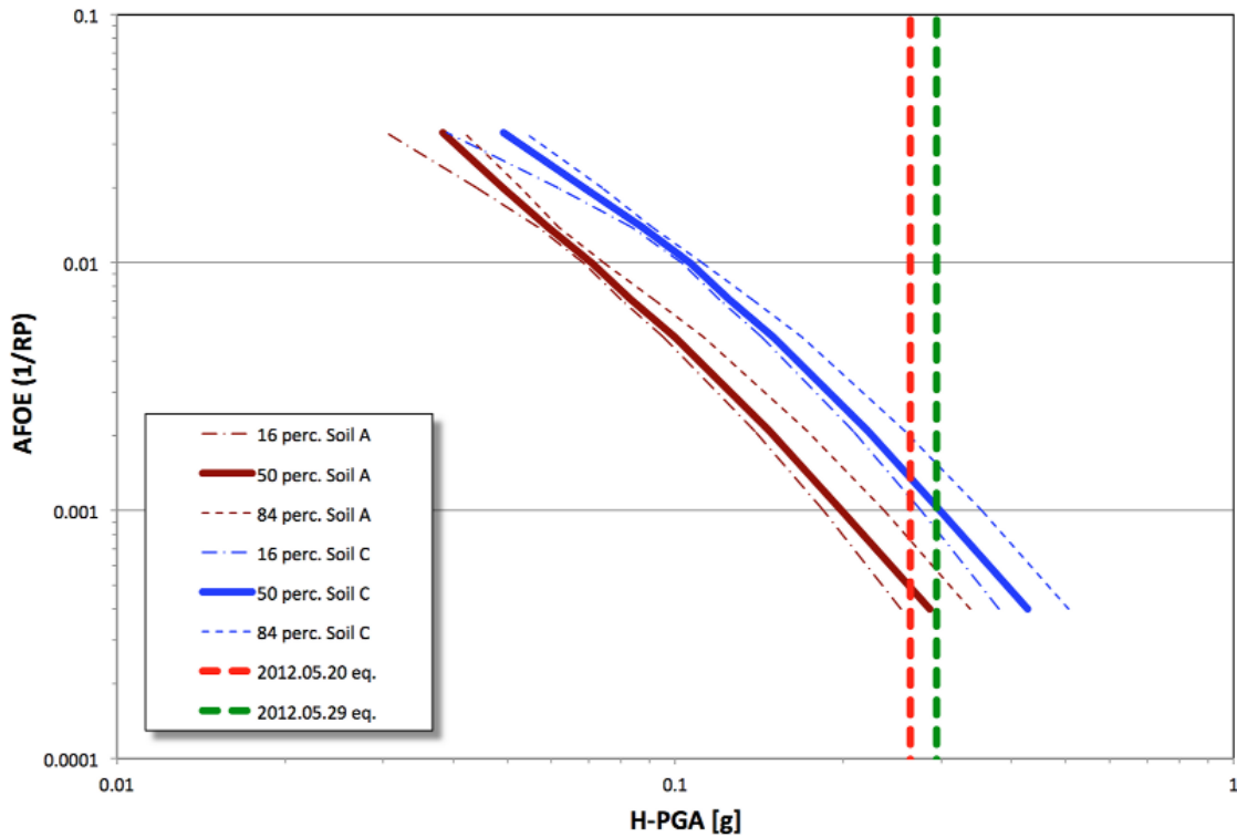
Figure 6. Comparison between the hazard curves for soil types A and C, computed at the node of the computational grid closest to Mirandola and the maximum horizontal PGAs recorded at the MRN station for the May 20 and 29, 2012, earthquakes. The 16th and 84th percentile curves represent the epistemic uncertainty of the probabilistic seismic hazard estimate.
