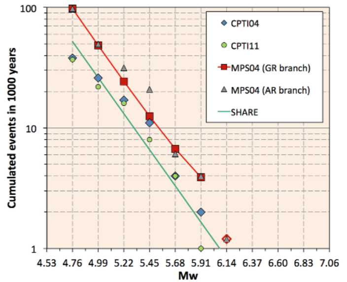
Figure 3. Comparison between the cumulative number of earthquakes in the CPTI04 and CPTI11 catalogs and the seismicity rates for the GR and AR branches of MPS04 and for the SHARE project (as available on July 2012) for seismic source zone 912. All rates are normalized to 1000 years.
