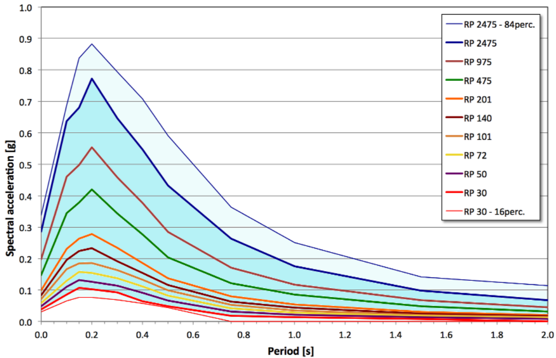
Figure 4. Acceleration uniform hazard spectra for several return periods (as indicated) considered in MPS04 at the grid point closest to the Mirandola (MRN) station.
