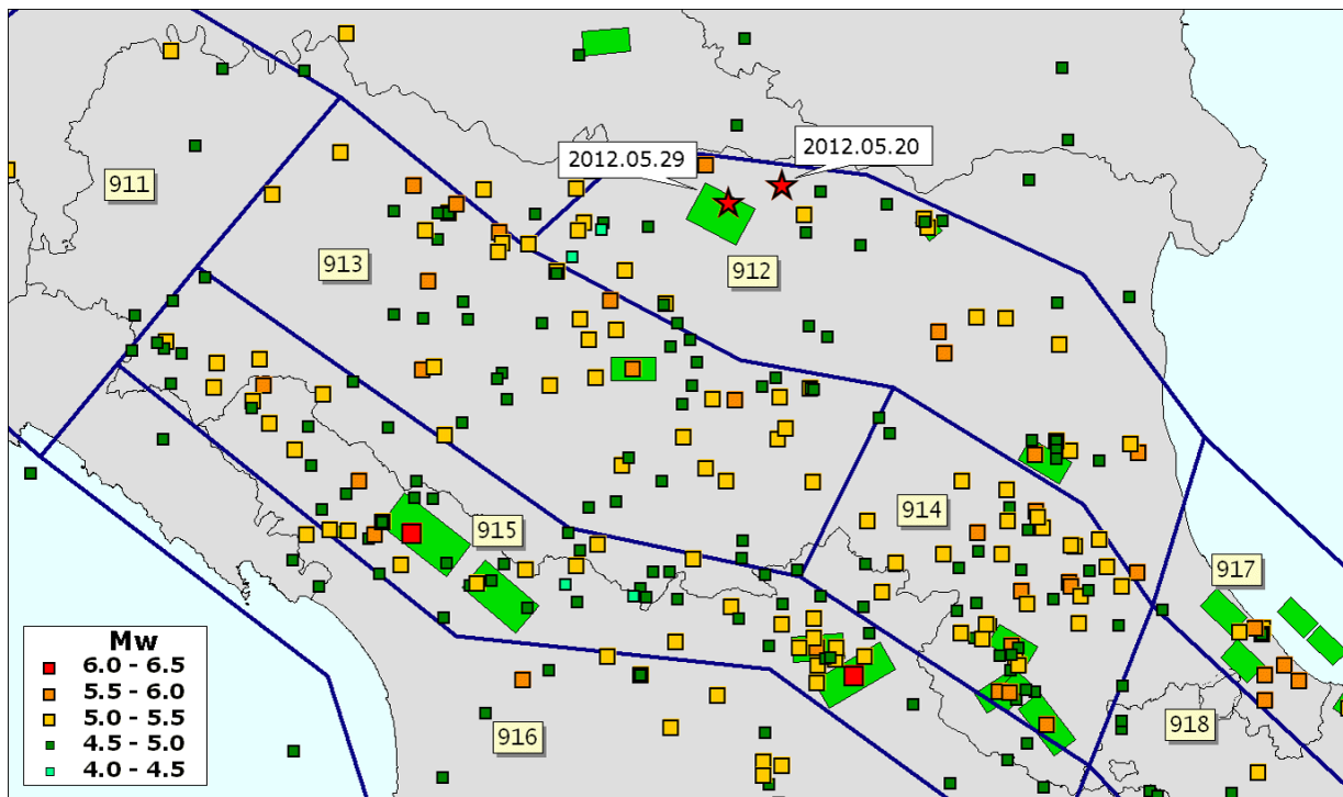
Figure 2. Seismic source zones from the ZS9 model (blue lines), potential seismogenic structures from the DISS database (green boxes), and earthquakes from the CPTI04 catalog (magnitudes mainly derived from historical data) in the northern Apennines. Red stars, epicenters of the two main events of the Emilia earthquake sequence.
