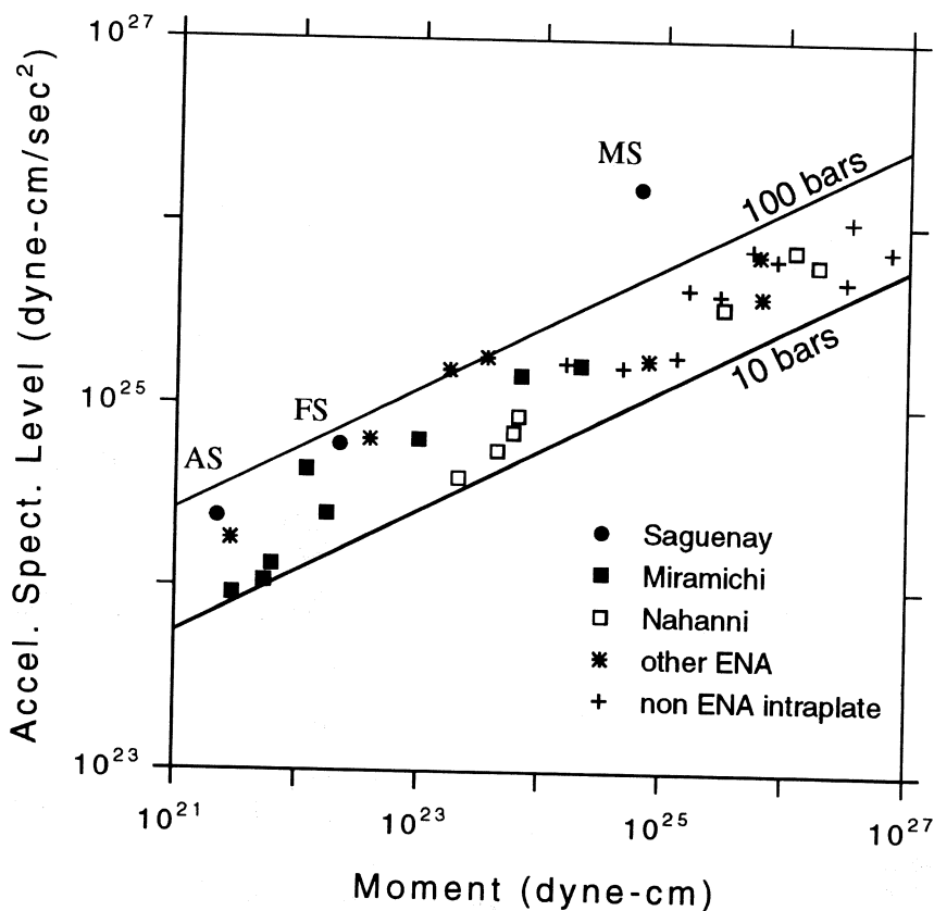
Fig. 6. Scaling of high frequency source spectral level for intraplate events (from Boore and Atkinson, 1992).
