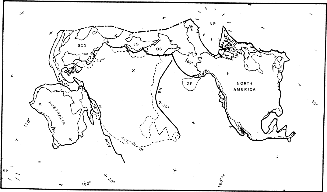
Fig. 2. Conformities and arrangement symmetry continent-basin and viceversa in Northern Hemisphere. North America corresponds in shape to Western Pacific. Juan de Fuca plate corresponds in shape to New Britain ovoidal plate. Solid lines represent coast contour. Bold lines represent major tectonic discontinuities as continental shelves margins, trenches and spreading ridges. The broken bold line is an arbitrary boundary between Asia (not represented in figure) and East Asiatic trench arc zones. Dotted lines represent computer aided rotations of the North American continental shelves and Juan de Fuca plate contours. SCS = South China Sea; JS = Japan Sea; OS = Ochotsk Sea; ZF = Zodiac Fan; EH = Emperor Hawaii volcanic chain; JF = Juan de Fuca plate; NB = The little New Britain ovoidal plate; MSV = Manus, Salomon, Vityaz trenches; NP = North Pole; SP = South Pole.
