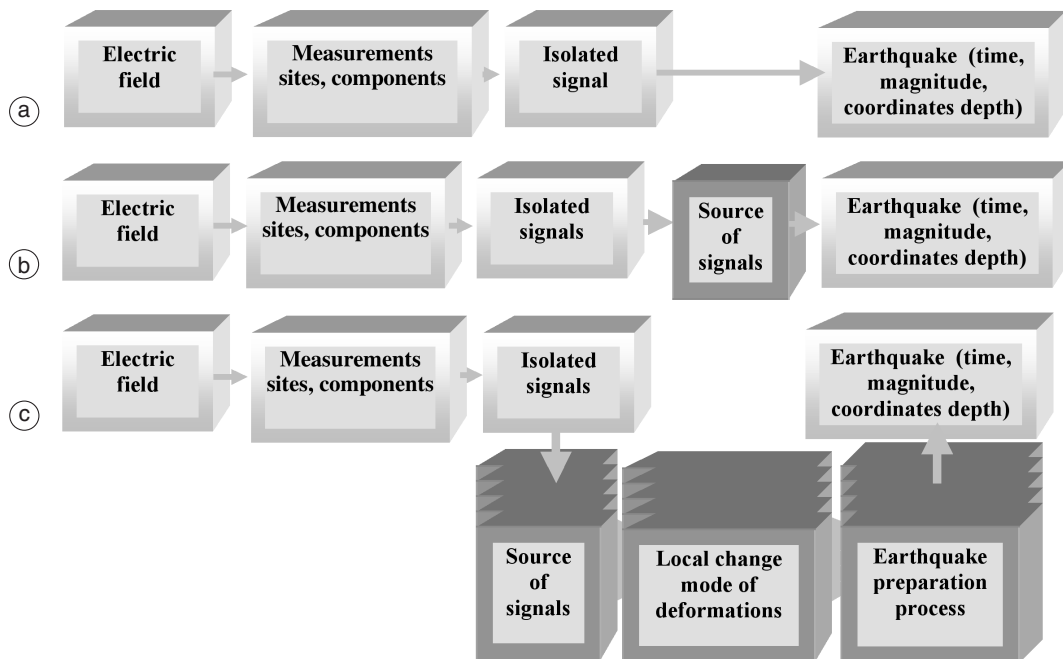
Fig. 11a-c. a) Standard and (b) new proposed empirical schemes of the forecast. c) The so-called theoretical scheme is also presented in the figure (see text).
