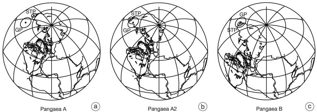
Fig. 1a-c. Comparison of Gondwana mean palaeopole (GP) for 250±10 Ma and Siberian Trap mean palaeopole (STP) in different Pangaea reconstructions with Central Africa held fixed at present geographic coordinates. a) Pangaea A model, notice the discrepancy between the mean palaeopoles. b) Pangaea A2 model, the mean palaeopoles are indistinguishable at 95% of confidence level, although there is a great circle distance of about 9° between them. c) Pangaea B model, the mean palaeopoles get the better fit. A supposed mega-shear of about 3700 km is required to pass from this Pangaea configuration to a Pangaea A model (the starting point of the break up of this super-continent during Middle Jurassic time).
