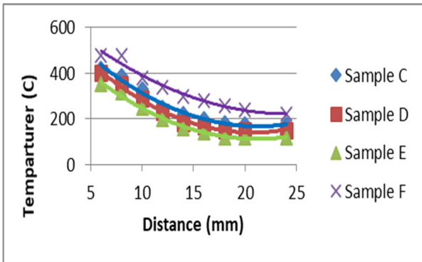
Fig. 6a. Distribution of temperature on surface for specimens (C,D,E,F).
