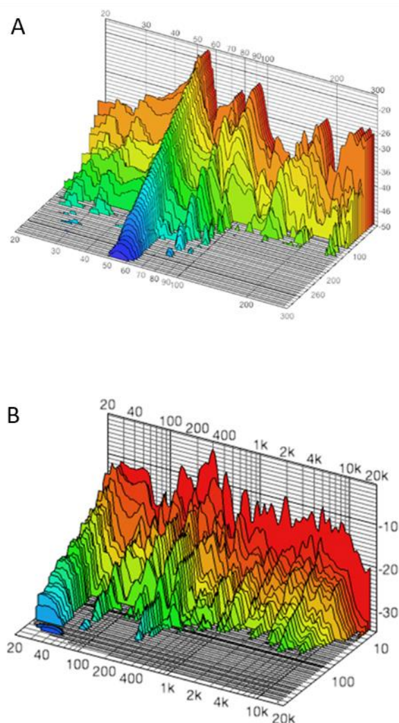
Figure 2 3D Simulation of (A) FT-IR spectrum and (B) Raman spectrum of Saxitoxin (STX).
