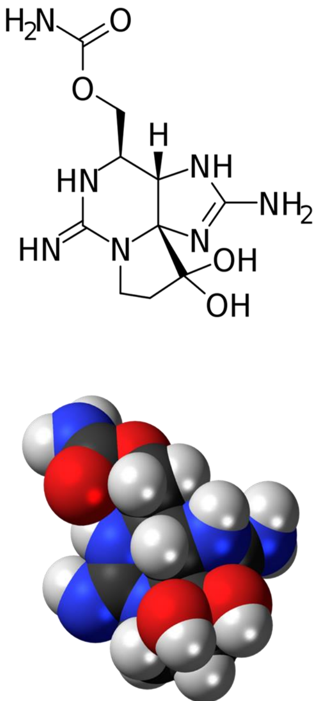
Figure 1 Different sections of the Saxitoxin (STX) [1–93].
