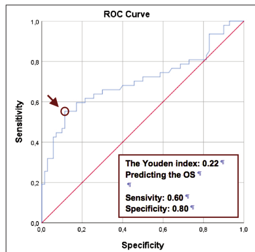
Figure 1. ROC curve.
