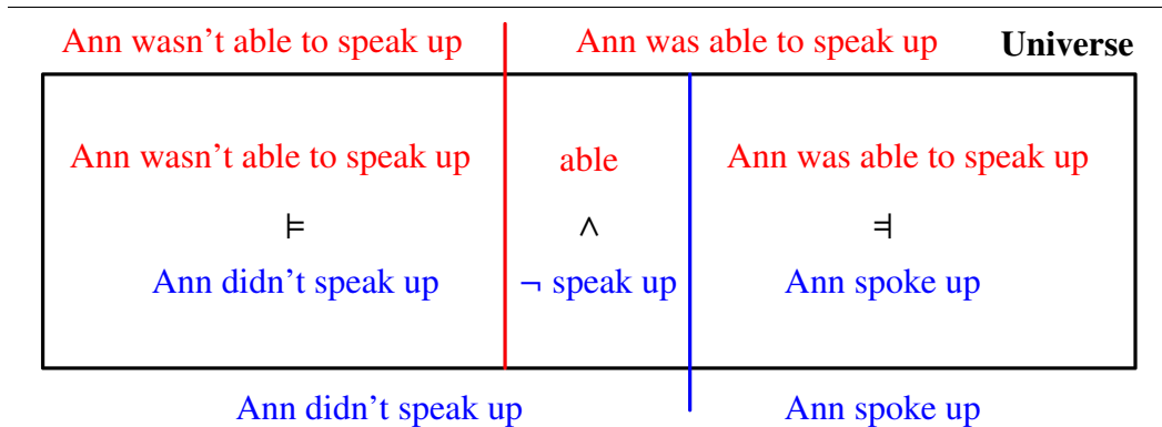
Figure 1 A cover relation: Ann was able to speak up \sim Ann didn't speak up
