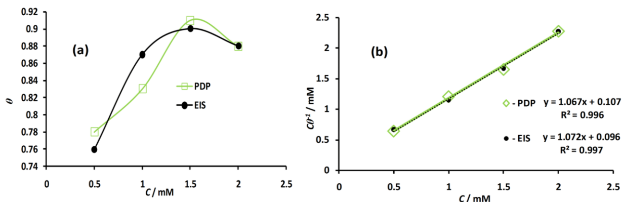
Figure 6. (a) Plot of concentration of DCH versus surface coverage and (b) Langmuir isotherm plot obtained for the adsorption of DCH on the surface of AA6061 in 3.5 % NaCl. [Symbols \square and \bullet represent the data points of PDP and EIS studies respectively, connected with trendlines]
