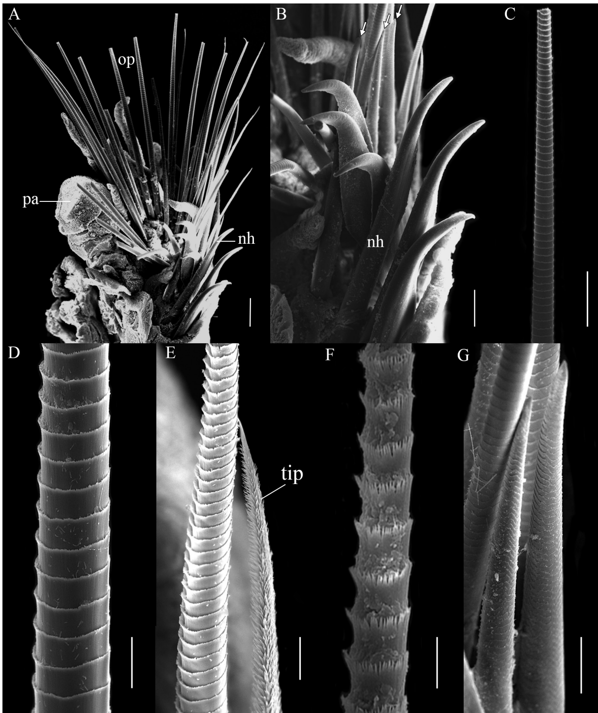
Fig. 7. Phalacrostemma danieli sp. nov., paratype (UMML-22.1181). A. Right opercular lobe. B. Nuchal hooks. C–D. Basal region of outer palea. E. Middle region and tip of outer paleae. F. Middle-distal region of outer palea. G. Inner paleae. Abbreviations: nh = nuchal hooks; op = outer paleae; pa = palps; tip = outer palea tip. Arrows indicate inner paleae. Scale bars: A = 200 \mu m; B–C = 100 \mu m; D = 20 \mu m; E, G = 50 \mu m; F = 10 \mu m.
