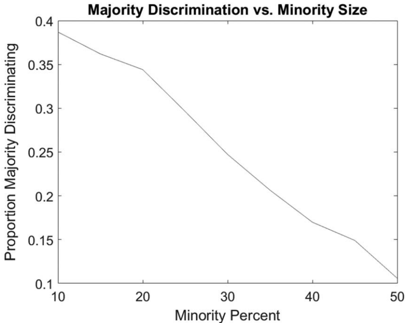
Figure 4. Level of majority discrimination, given by the percentage of the majority group whose out-group strategy is to demand High, with different sizes of minority groups. Color version available as an online enhancement.
